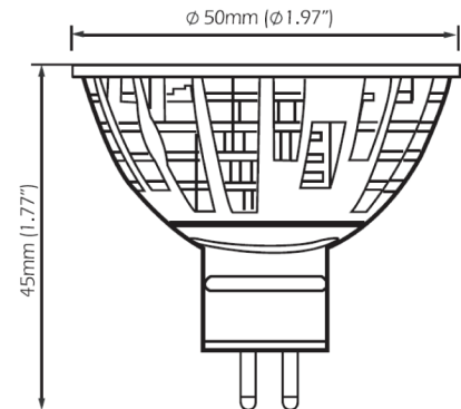
GU 5.3 Base
